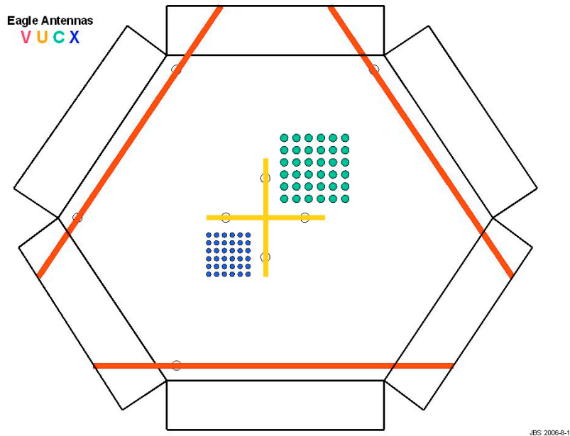
Figure 2 – Antenna Placement on 600 mm per side Hexagonal Spaceframe
