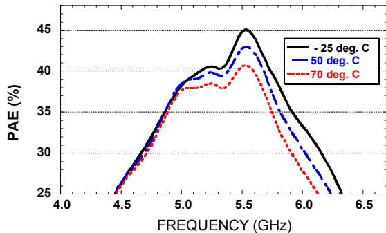
PAE, P_{IN} = +12 \text{ dBm} , V_{DD} = 7 \text{ V}
